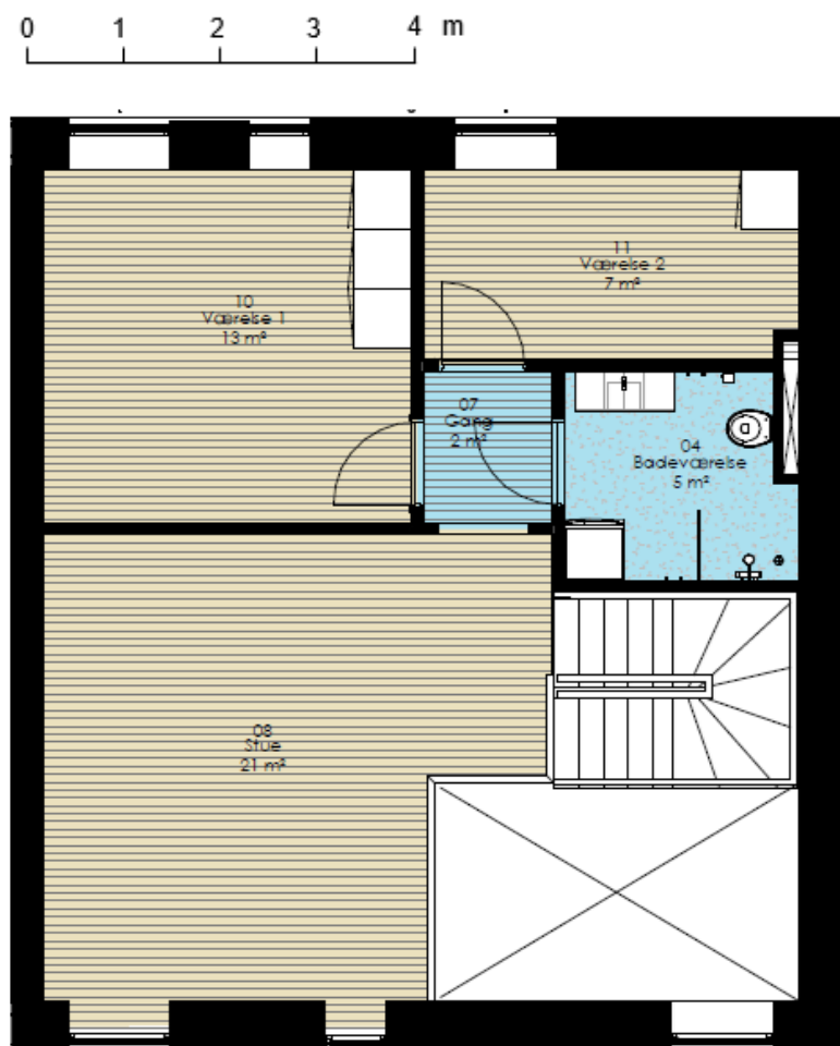
2. sal, 115 m²
