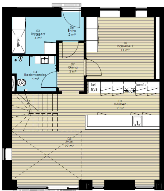
Stueplan, 109 m 2
